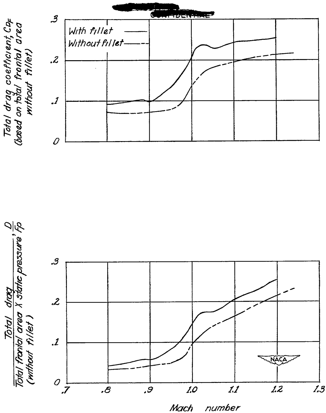
Figure 7.- Comparative variations with Mach number of drag coefficient and D/F_p for the wing-body configuration with wing fillet and without wing fillet.
