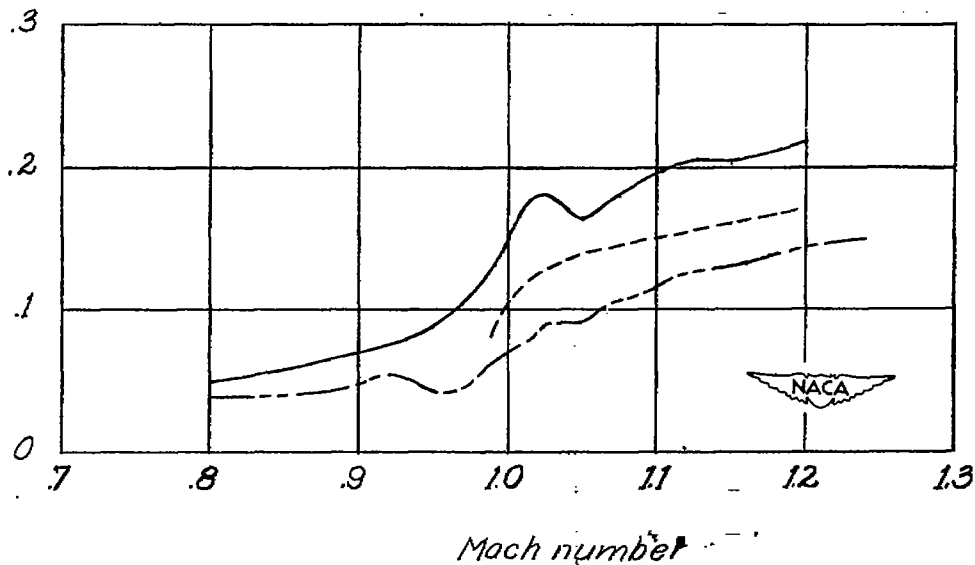
Figure 10.- Comparative variations with Mach number of drag coefficient and D/F_p for the body of the wing-body configuration with wing fillet and without wing fillet. CONFIDENTIAL
