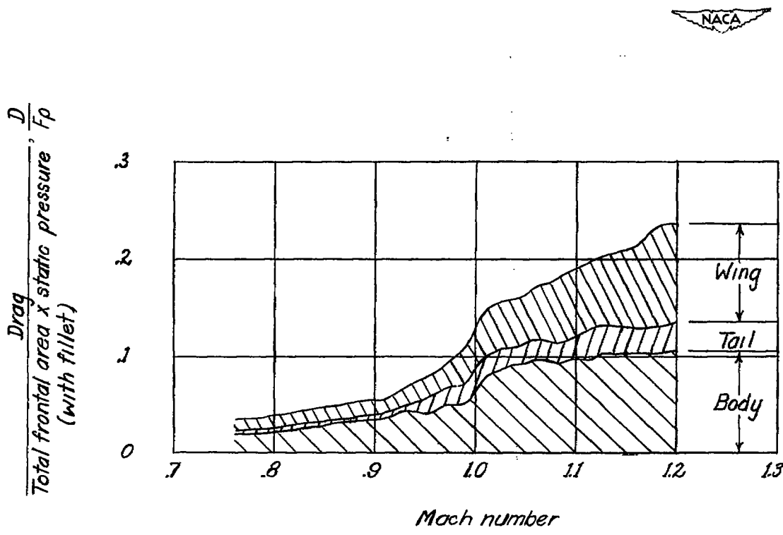
Figure 6.- Variation with Mach number of drag coefficient and D/F_p for the wing-body configuration with wing fillet.
