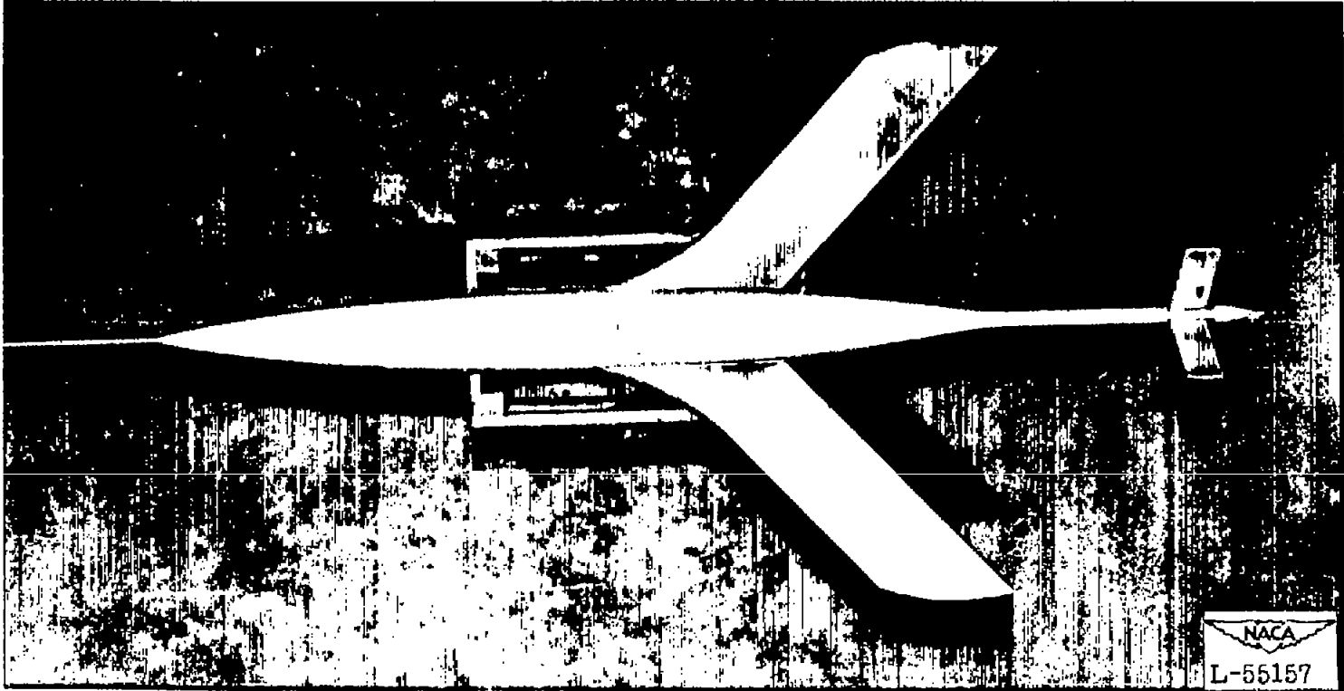
Figure 2.- Top plan view of wing-body combination with wing fillet.
