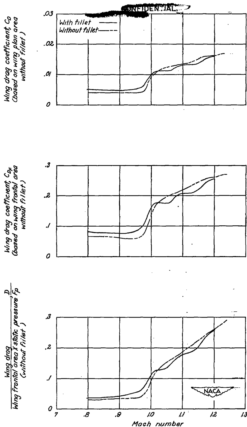
Figure 8.- Comparative variations with Mach numbers of drag coefficients and D/F_p for the wing of the wing-body configuration with wing fillet and without wing fillet. CONFIDENTIAL
