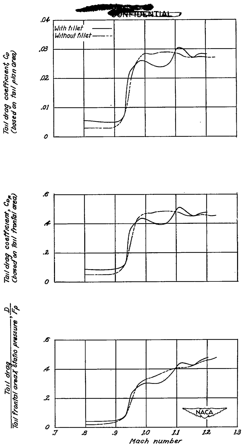
Figure 9.- Comparative variations with Mach number of drag coefficients and D/F_p for the tail fins of the wing-body configuration with wing fillet and without wing fillet. CONFIDENTIAL
